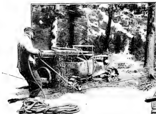
By means of caterpillar-type wheels, a portable bridge and a drum-and-rope device for crossing turbulent streams the trail was covered in two days
